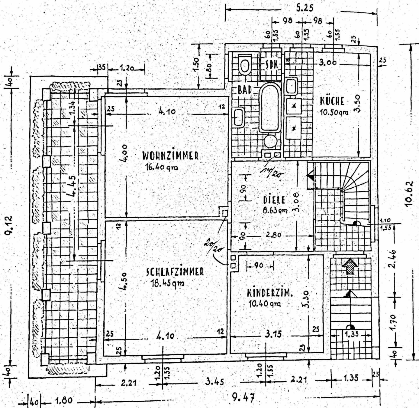
ERDGESCHOSS.
